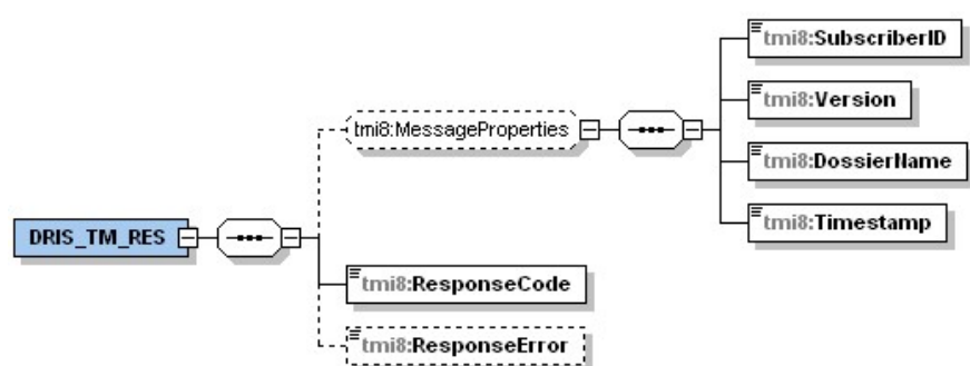
Figuur 15 XSD DRIS_TM_RES
