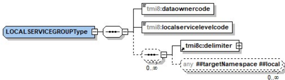
Figuur 21 XSD LOCALSERVICEGROUP
