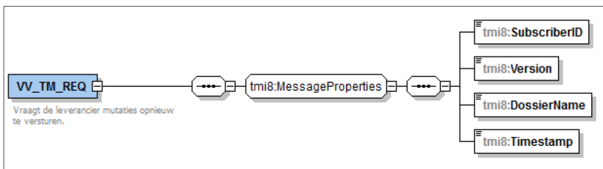
Figuur 11 XSD VV_TM_REQ
