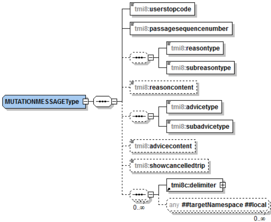
Figuur 23 XSD MUTATIONMESSAGE
