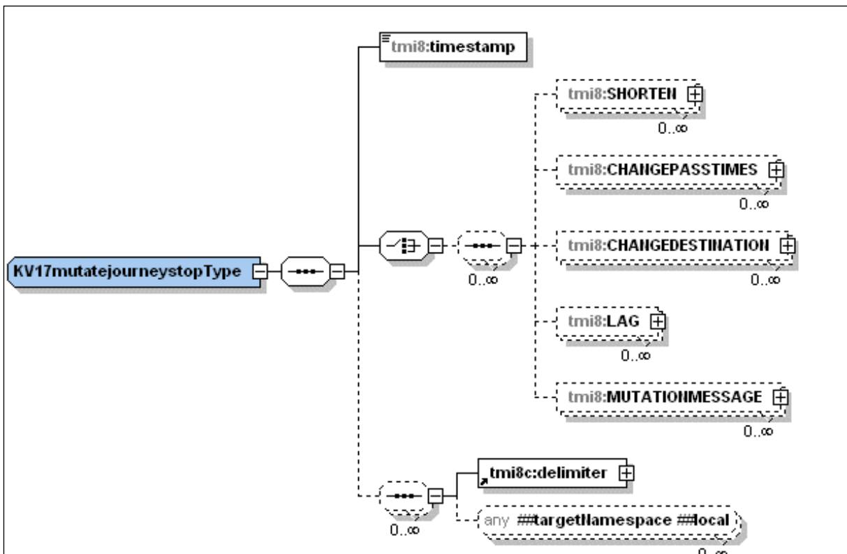
Figuur 16 XSD KV17MUTATEJOURNEYSTOP
