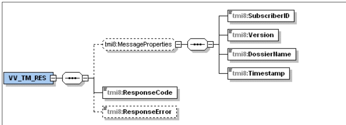
Figuur 12 XSD VV_TM_RES
